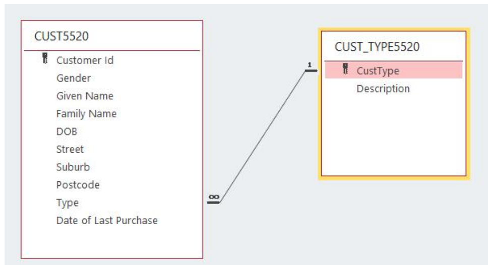
Figure 5: Relationship between CUST5520 and CUST_TYPE5520 Tables.
