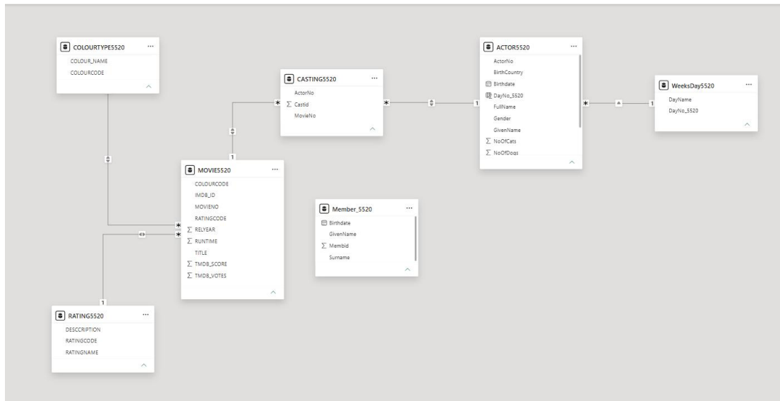
Figure 25: Relationships View of the Database Model
